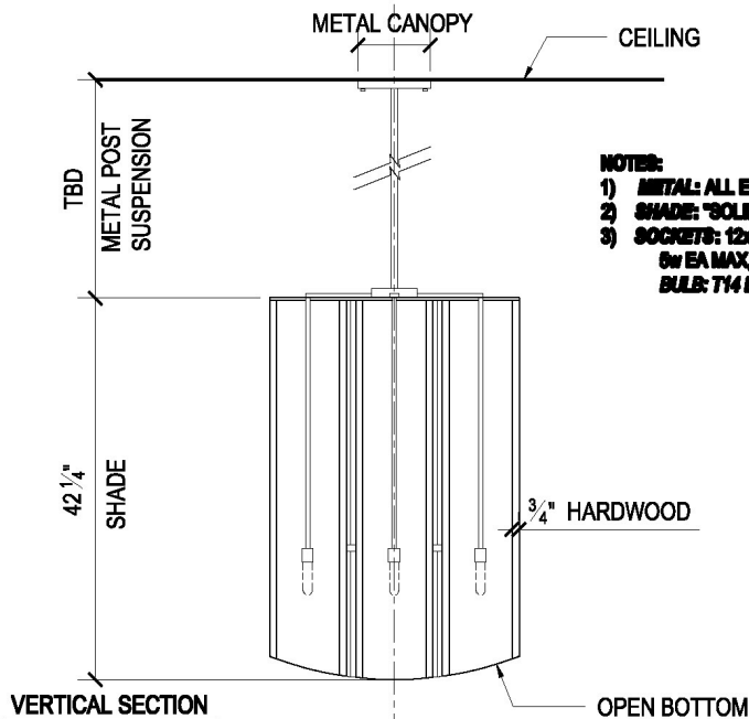
VERTICAL SECTION
