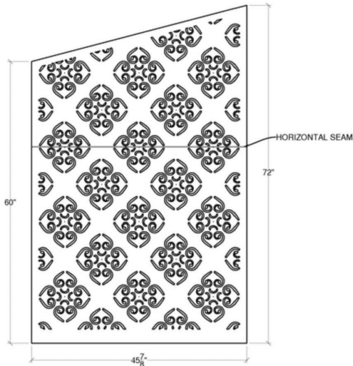
FLATTEN PATTERN SIDE VIEW
